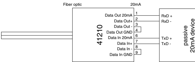
Interface Tx and Rx loop active
